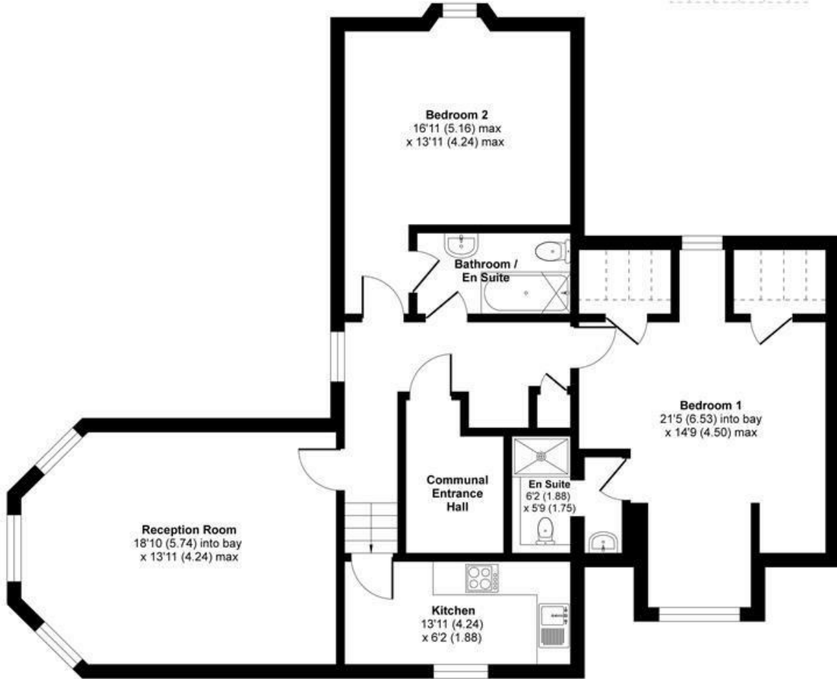
SECOND FLOOR
